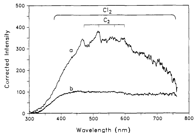
Figure 9. Sonoluminescence spectra of halocarbons: (a) SL from tetrachloroethylene under Ar at 0 °C, vapor pressure = 4.1 Torr. Spectrum is the concatenation of three spectra, each the average of three 100-s spectra. (b) SL from \text{CCl}_4 under Ar at -7 °C, vapor pressure = 23 Torr. Spectrum is the concatenation of three spectra, each the average of 20 100-s spectra.
